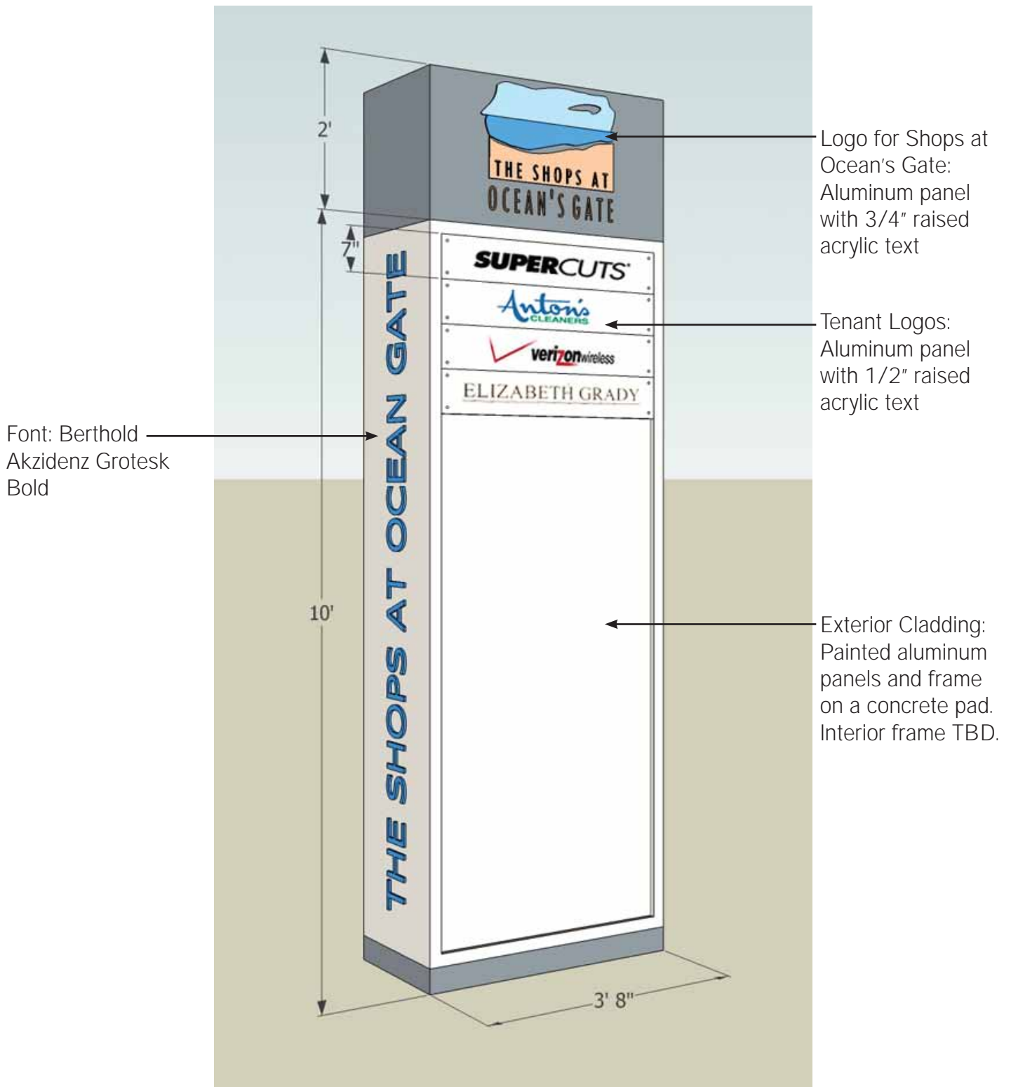
Dimensions of Pylon = 12' H x 3'-8" W x 2' D
